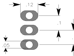
TO-220-3
