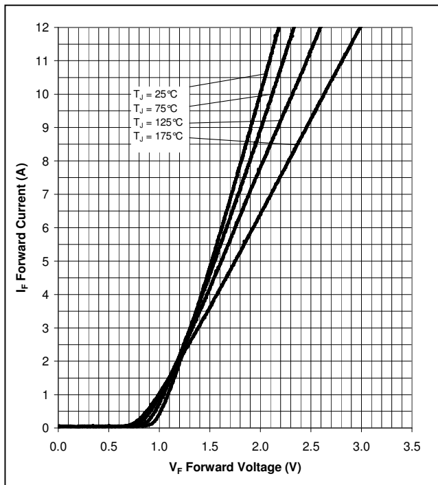
Figure 1. Forward Characteristics
