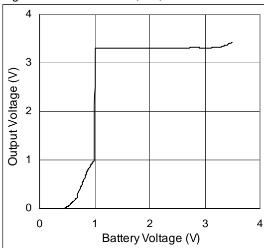
Figure 6. V_{OUT} vs. V_{BATT} ; Shutdown, No Load
