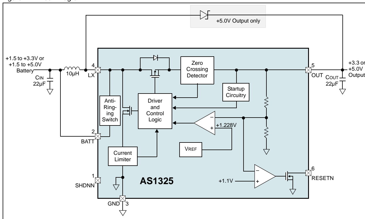
Figure 27. Block Diagram
