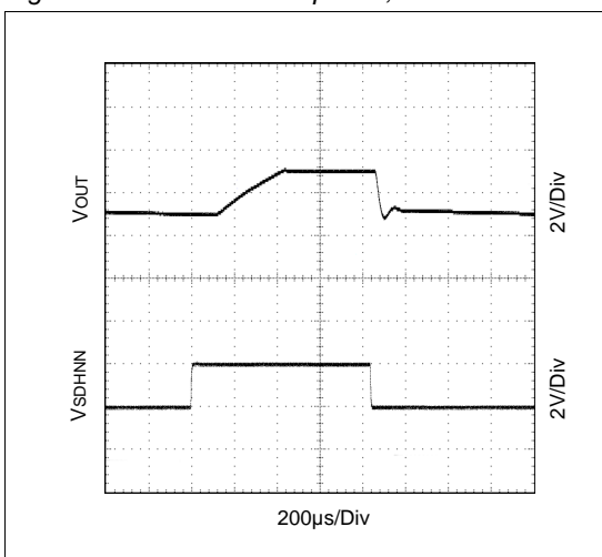
Figure 24. Shutdown Response; R_{LOAD} = 100\Omega
