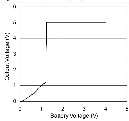
Figure 18. V_{OUT} vs. V_{BATT} ; Shutdown, No Load
