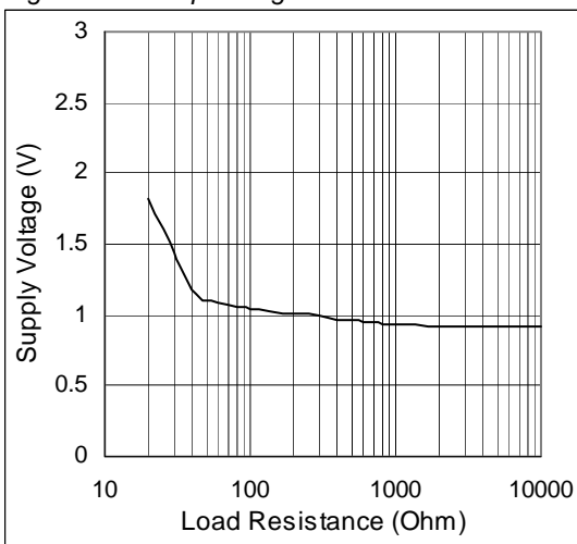
Figure 8. Startup Voltage vs. Load Resistance
