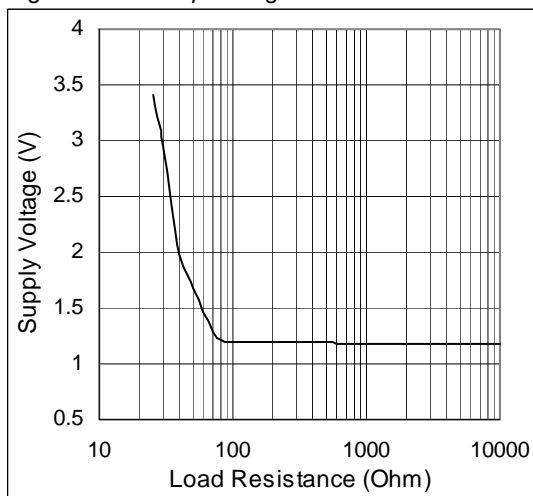
Figure 20. Startup Voltage vs. Load Resistance
