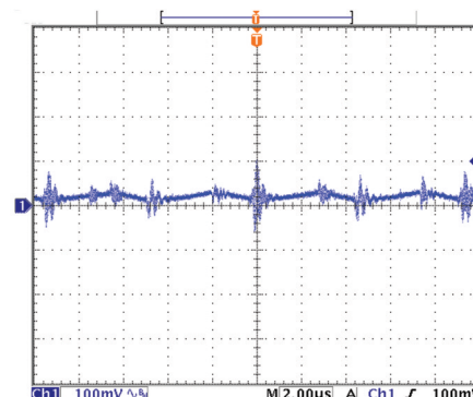
Figure 4 - V1 HPD1K5PS24 (Full load) 160mV pk-pk ripple and noise 20 MHz bandwidth
