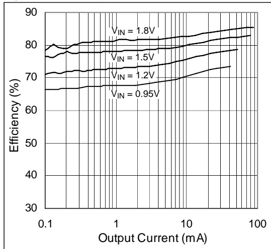
Figure 5. Efficiency vs. Output Current; V_{OUT} = 2.7V
