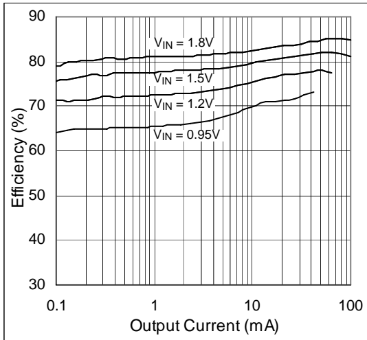
Figure 4. Efficiency vs. Output Current; V_{OUT} = 3.0V
