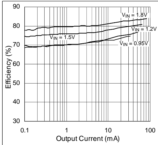
Figure 3. Efficiency vs. Output Current; V_{OUT} = 3.3V
