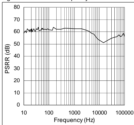
Figure 10. PSRR vs. Frequency
