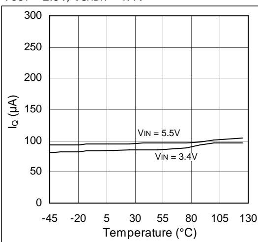
Figure 10. Quiescent Current vs. Temperature; V_{OUT} = 2.9\text{V} , V_{SHDN} = 1.4\text{V}
