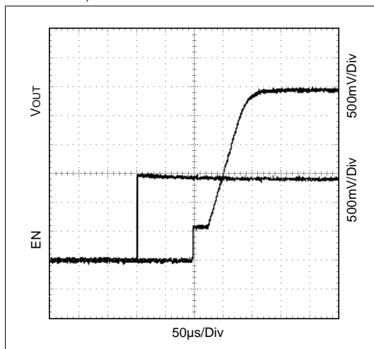
Figure 12. Turn On Time; V_{IN} = 3.3V , C_{BYPASS} = 10nF , C_{IN} = C_{OUT} = 1\mu F (Ceramic), t_R = 20ns , I_{OUT} = 1mA , V_{OUT} = 2.8V
