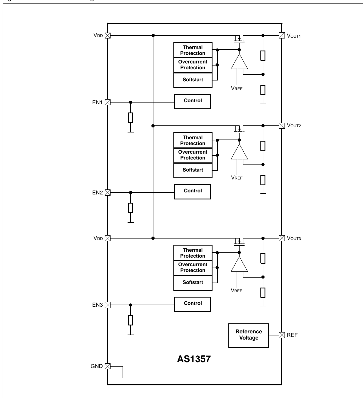
Figure 2. AS1357 Block Diagram
