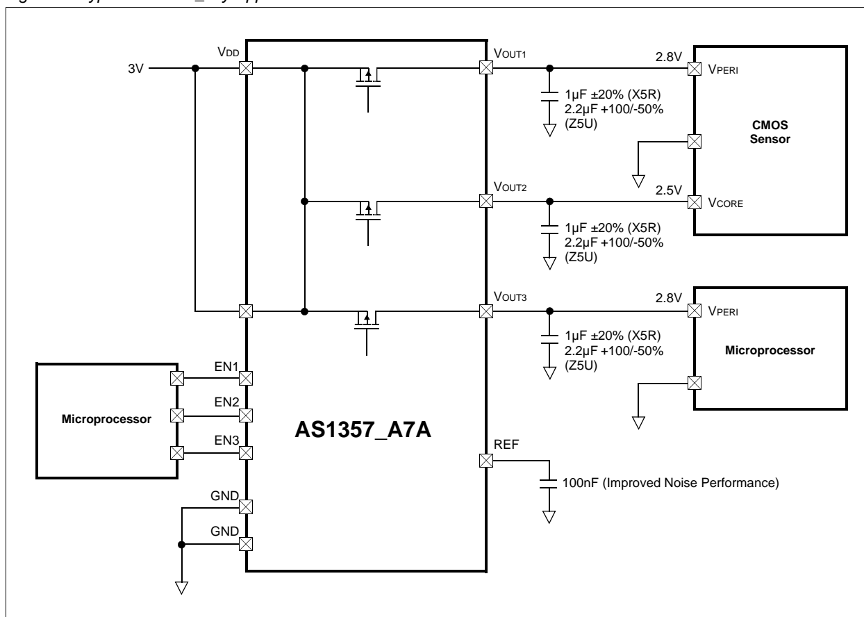
Figure 4. Typical AS1357_uxy Application
