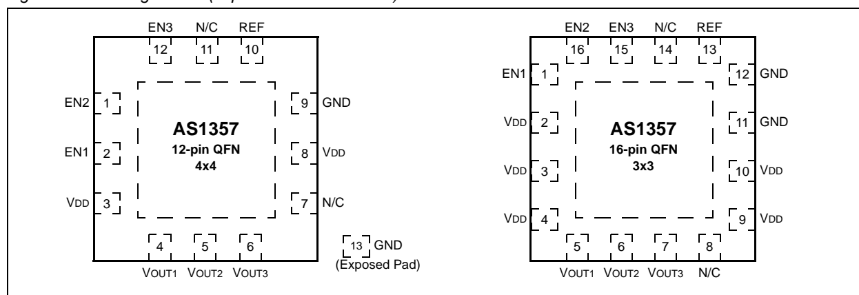
Figure 3. Pin Assignments (Top View – Not To Scale)
