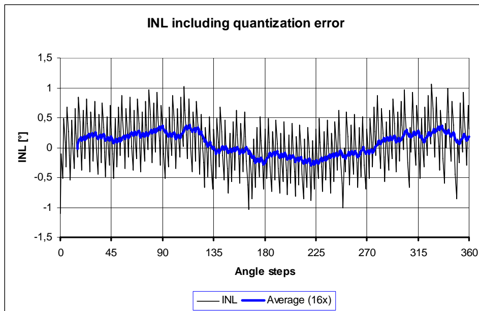
Figure 20: typ. INL error over 360°
