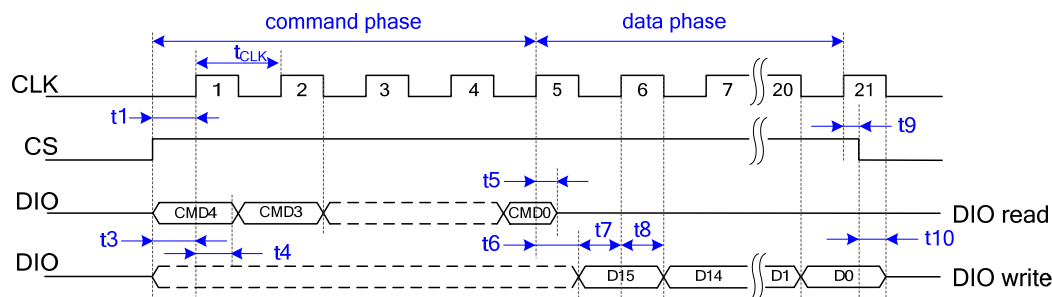
Figure 4: SSI read/write serial data transmission
