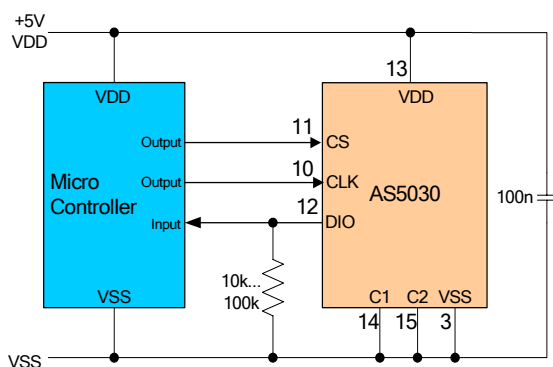
Figure 5: SSI read-only serial data transmission
