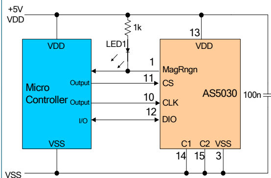
Figure 15: Magnetic field strength indicator
