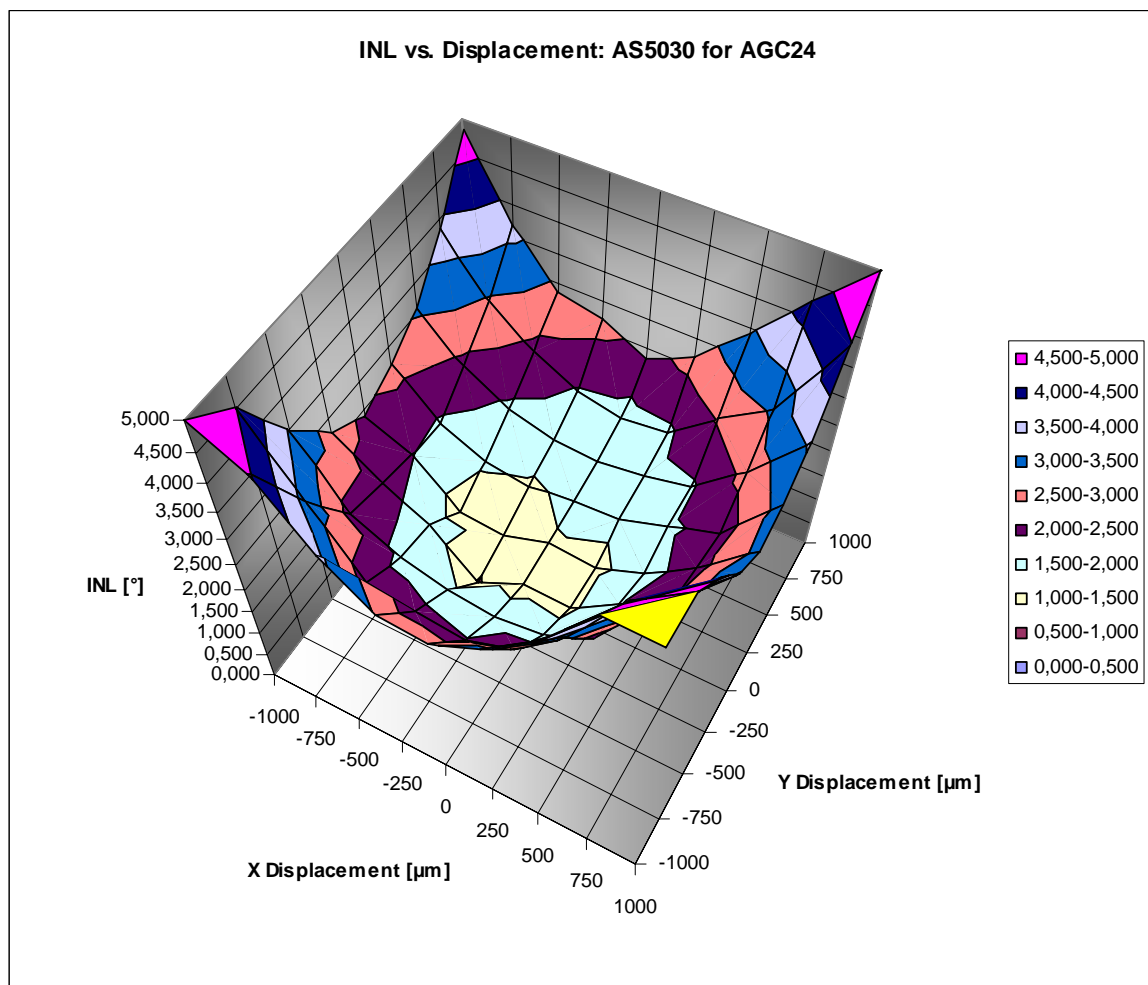
Figure 25: Typical error curve of INL error over lateral displacement (including quantization error)
