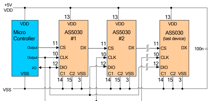
Figure 11: Connection of devices in Daisy Chain mode
