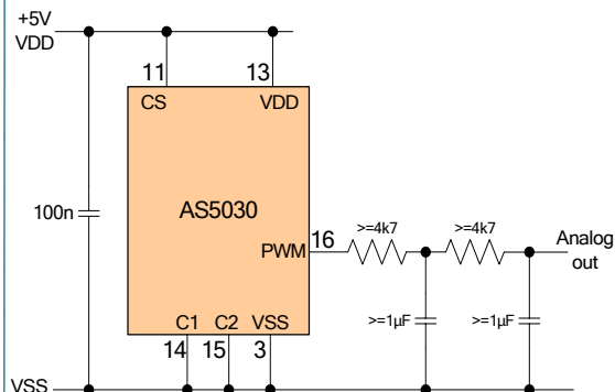
Figure 9: Data transmission with pulse width modulated (PWM) output
