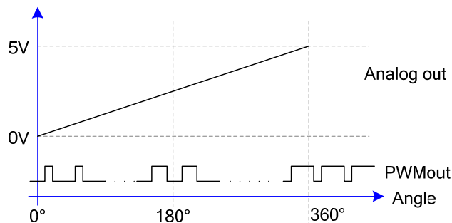
Figure 9: Data transmission with pulse width modulated (PWM) output
