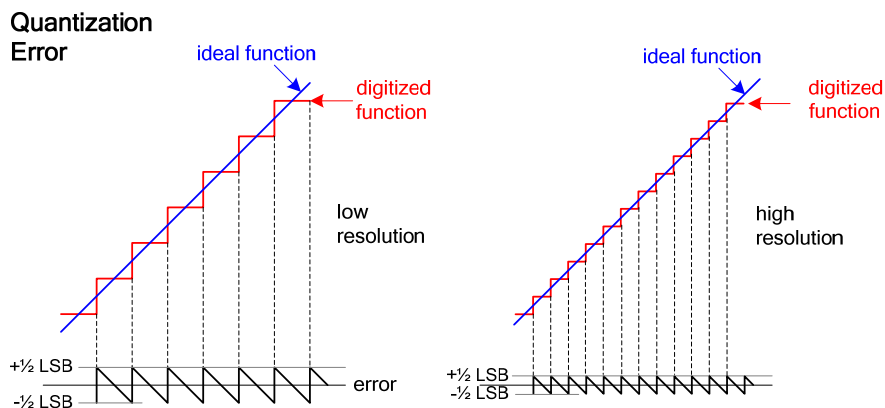
Figure 19: Quantization error of a low resolution and a high resolution system
