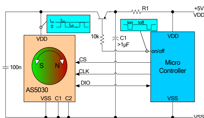
Figure 17: Application example III: ultra-low power encoder
