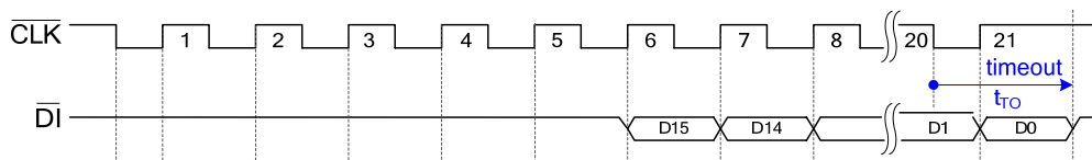
Figure 7: 2-wire SSI read-only mode
