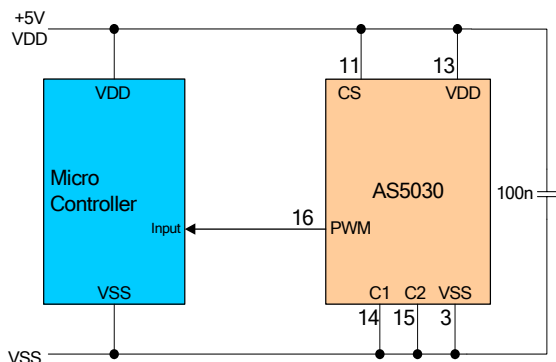
Figure 8: Data transmission with pulse width modulated (PWM) output
