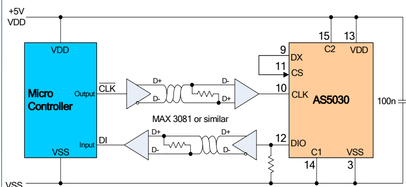
Figure 7: 2-wire SSI read-only mode
