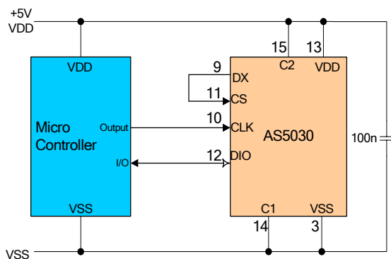
Figure 6: 2-wire R/W mode
