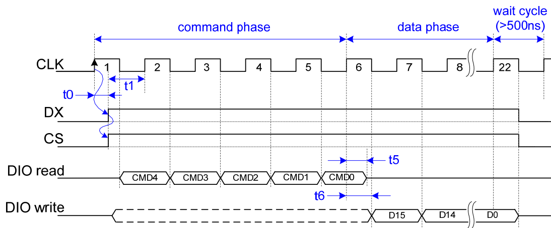
Figure 6: 2-wire R/W mode
