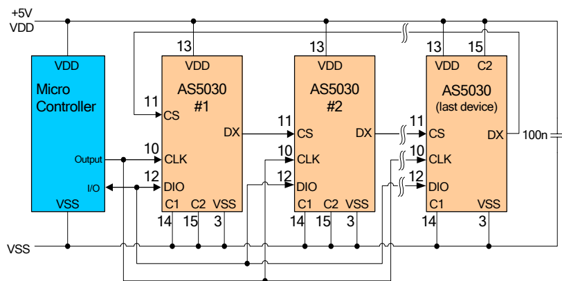
Figure 12: 2-wire Daisy Chain mode
