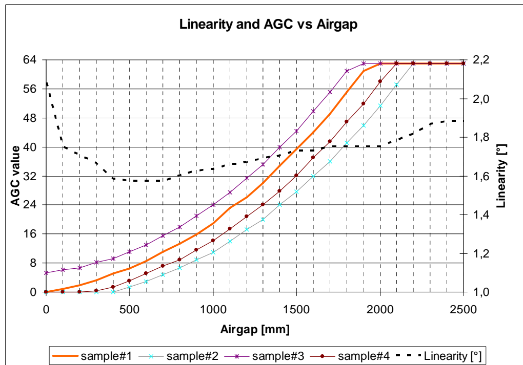
Figure 21: typical curves for vertical distance versus AGC value on several untrimmed samples
