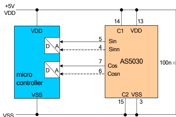
Figure 10: Sine and Cosine outputs for external angle calculation
