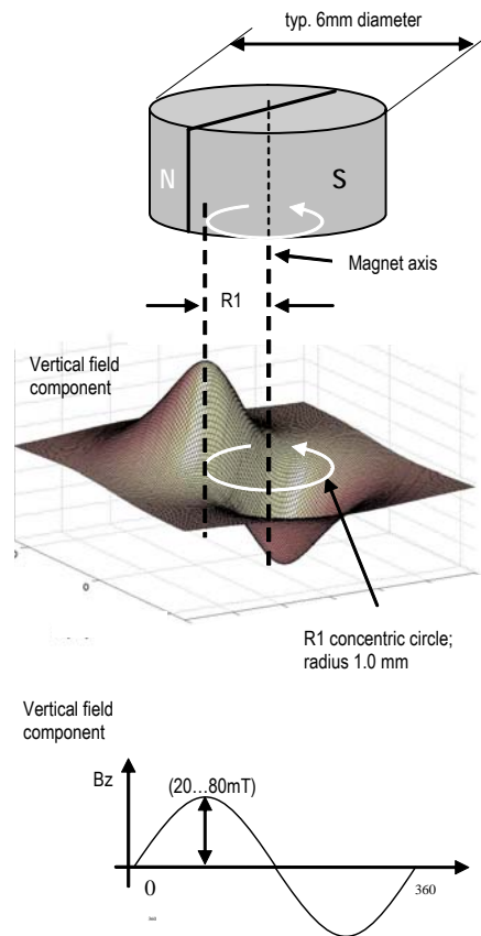
Figure 22: Vertical magnetic fields of a rotating magnet
