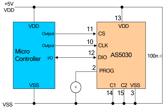
Figure 14: Analog OTP verification
