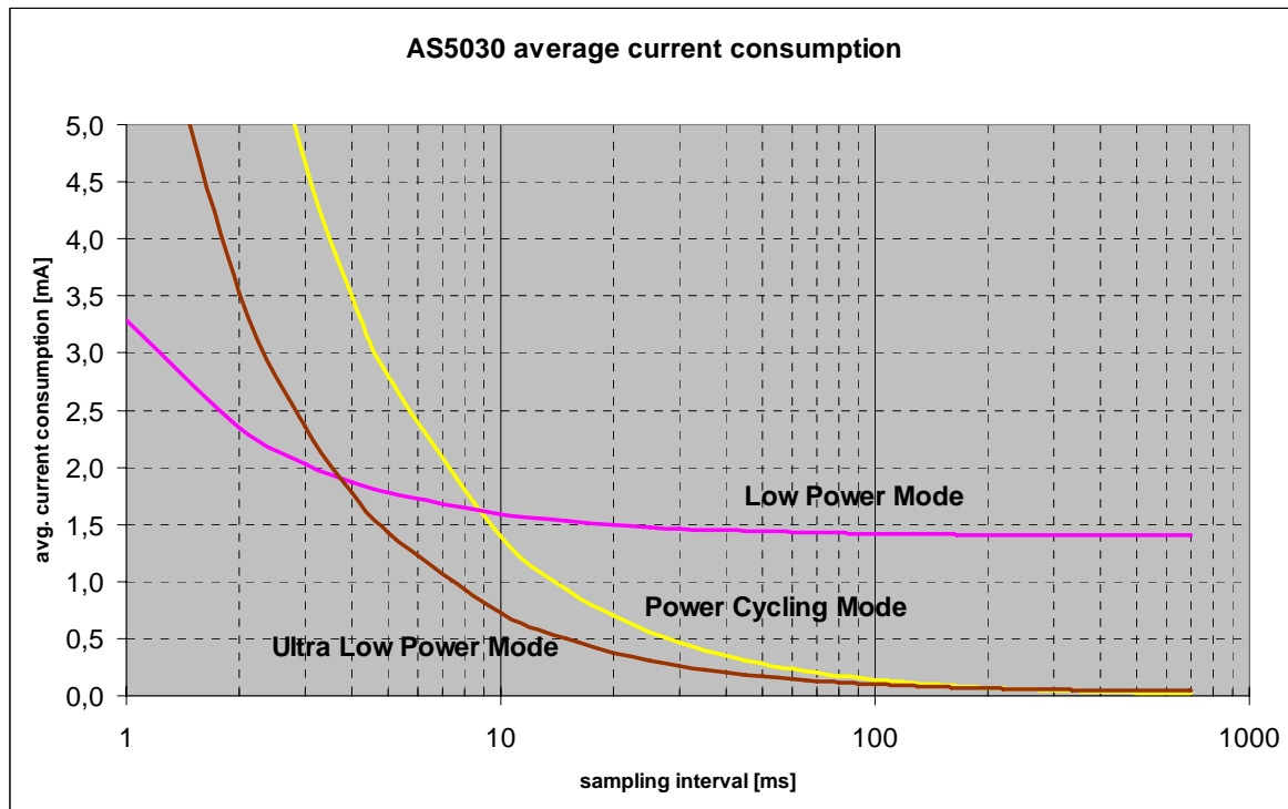
Figure 18: Average current consumption of reduced power modes
