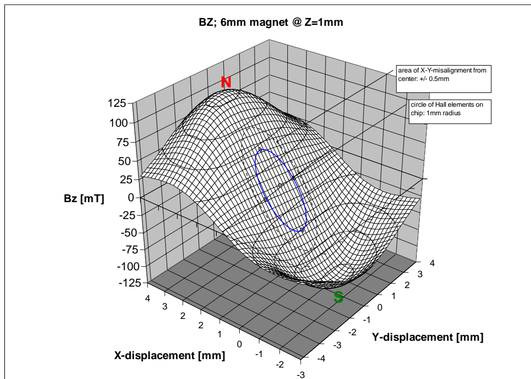
Figure 24: Vertical magnetic field distribution of a cylindrical 6mm \varnothing diametric magnetized magnet at 1mm gap
