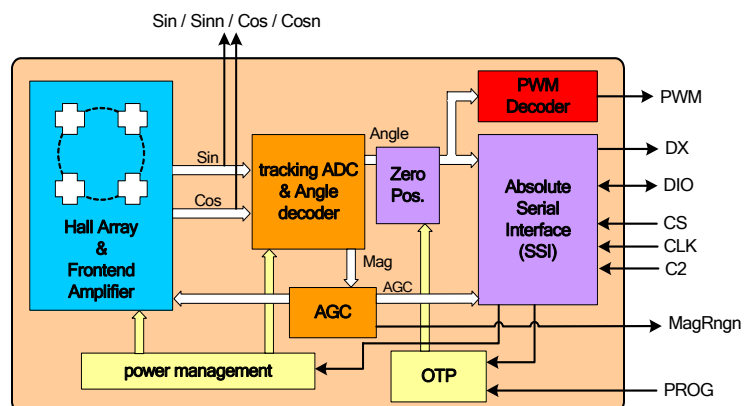
Figure 2: AS5030 block diagram
