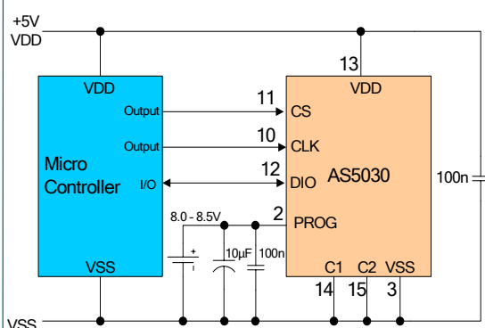
Figure 13: OTP programming connection
