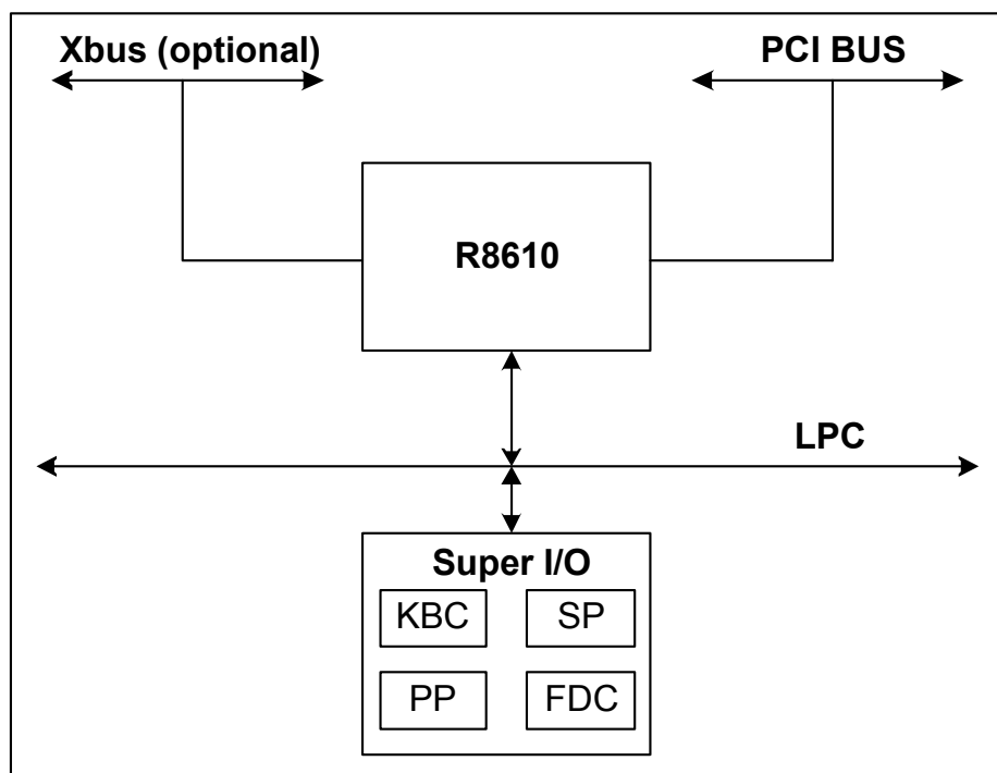
Figure 10-5. Typical Setup
