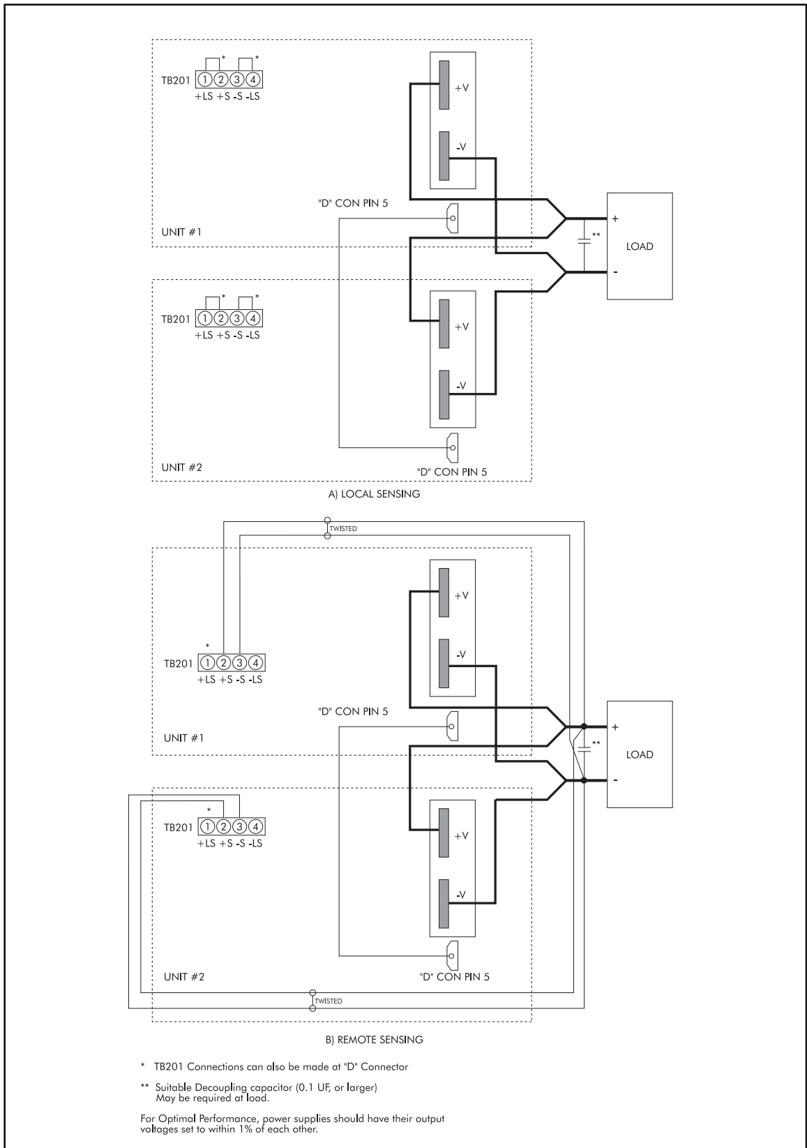
Figure 6 - Parallel Operation
