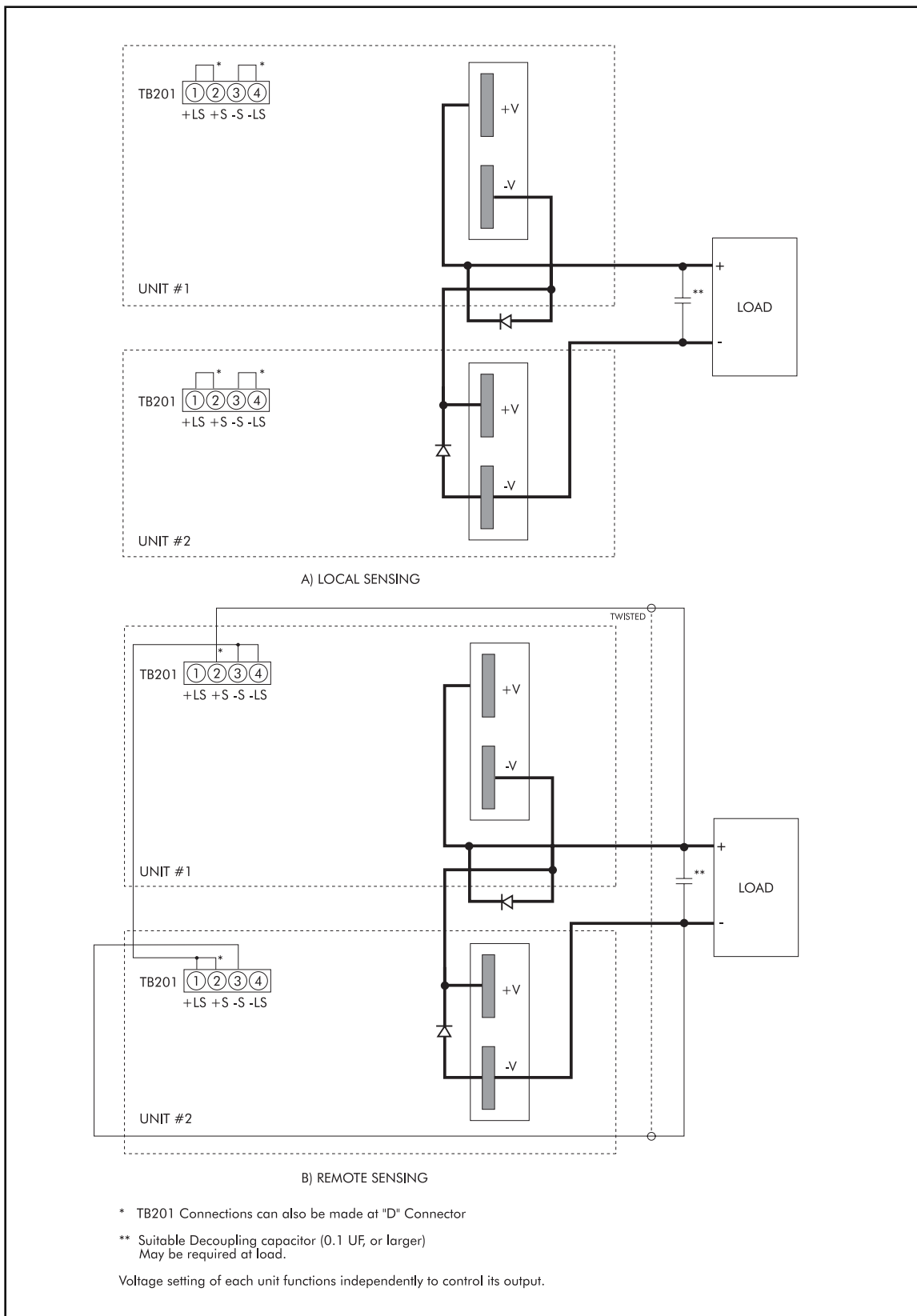
Figure 7 - Series Operation
