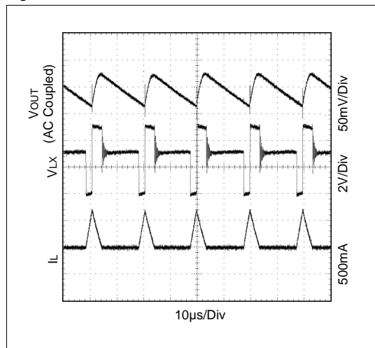
Figure 13. Waveforms; R_{LOAD} = 100\Omega , V_{BATT} = 3V
