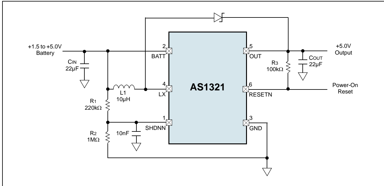
Figure 16. Low-Battery Cutoff Application Diagram
