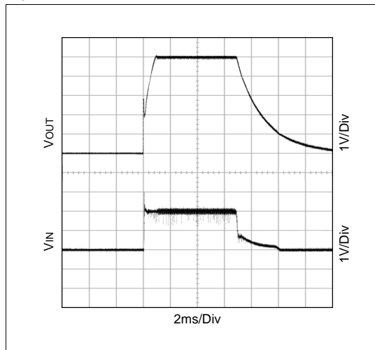
Figure 11. On/Off Response; R_{LOAD} = 100\Omega
