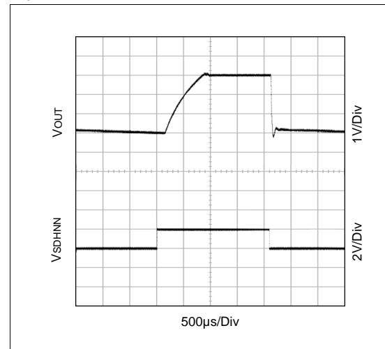
Figure 12. Shutdown Response; R_{LOAD} = 100\Omega
