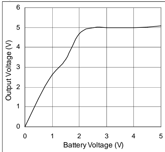
Figure 5. V_{OUT} vs. V_{BATT} ; Shutdown, 130mA Load
