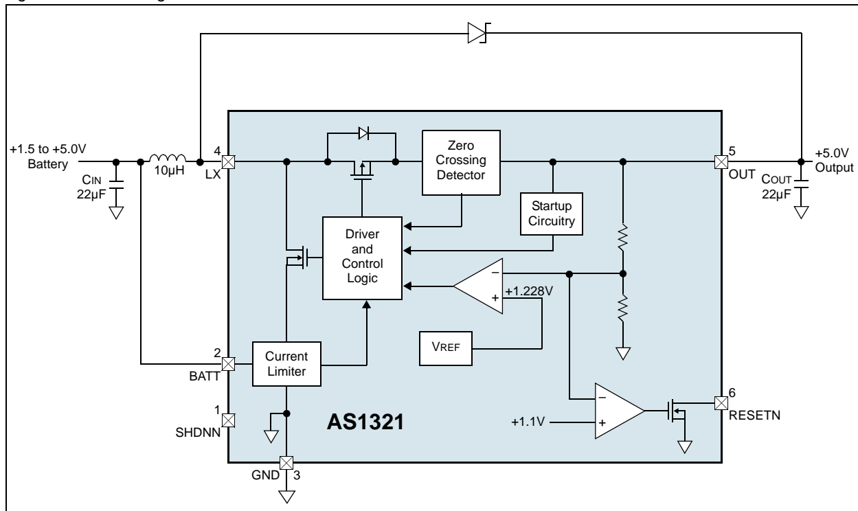
Figure 15. Block Diagram
