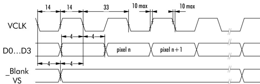
Figure 5. TFT mode. Minimum values in ns.
