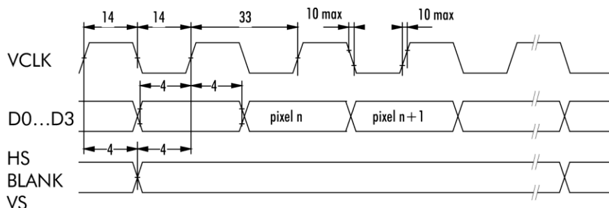
Figure 4. Normal and VGA mode. Minimum values in ns.
