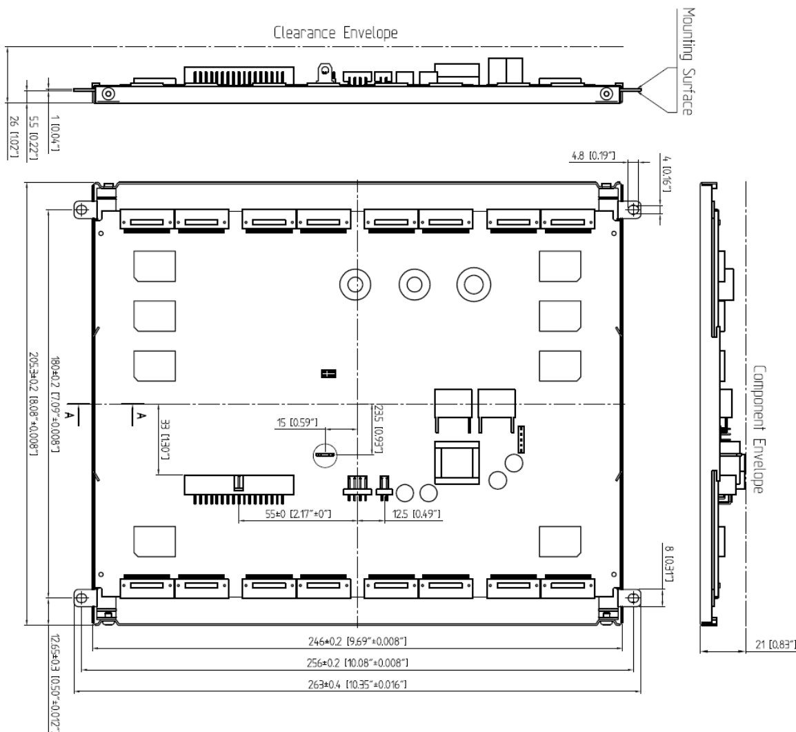
Figure 6. Mechanical dimensions. Dimensions are in millimeters; inches in brackets.
