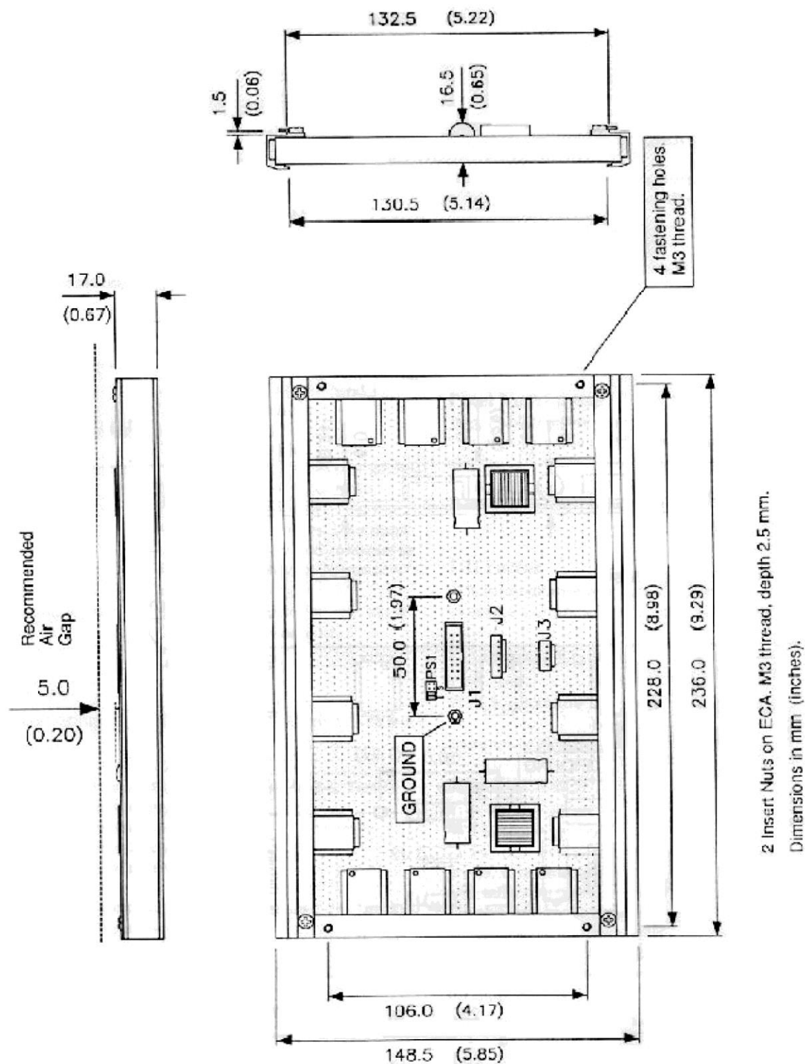
Figure 8. Back and side views with FRA aluminum mounting frame (dimensions in mm)
