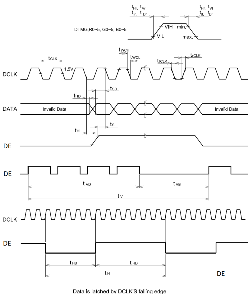
Figure 7. Timing chart
