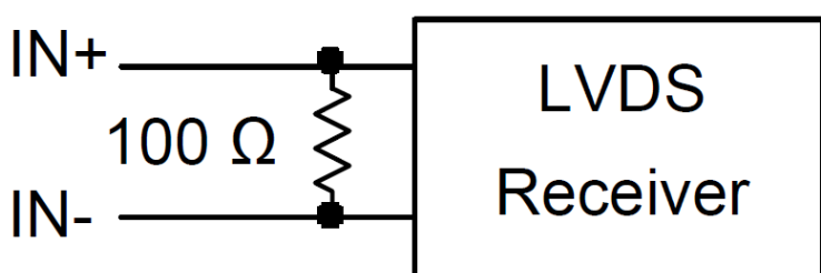
Figure 1. LVDS Input
